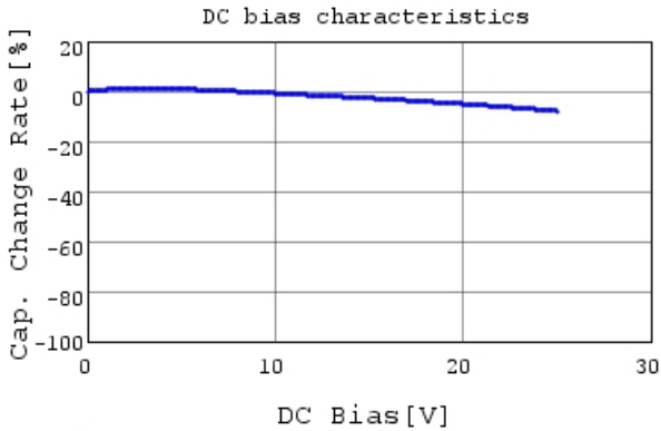
GCM188R71E103KA37 C-DC bias capchange, 25.0c
