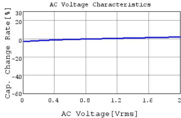
GCM188R71E103KA37 C-AC Voltage capchange, Dc
