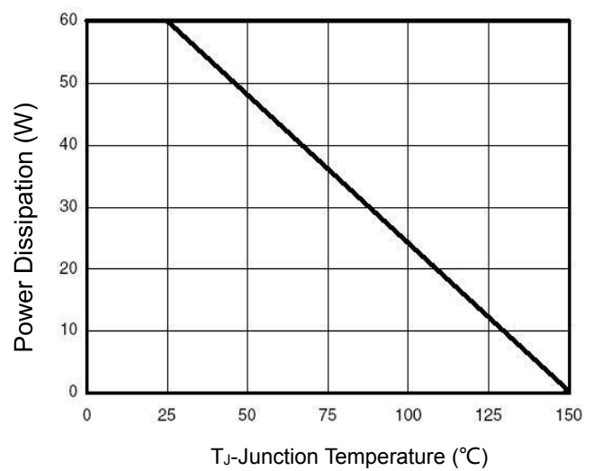
Figure 9 Power De-rating
