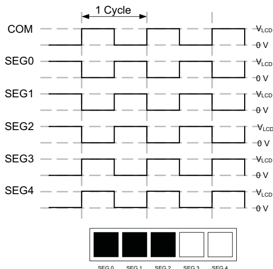
Figure 2-13. Static LCD Control Waveform
