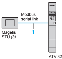
Example connection of an Altivar 32 drive and a Magelis STU HMI terminal via the Modbus serial link
