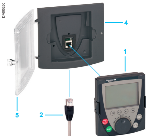
Using the graphic terminal in enclosure door: 1 + 2 + 4 (+ 5, if IP 65)
