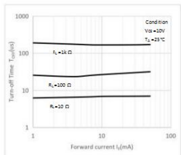
Fig 6. Turn-off Time vs Forward Current
