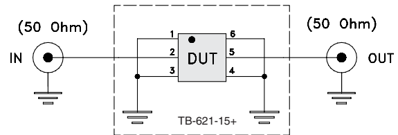
Fig 1. Block diagram of Test Circuit used for characterization, Test board TB-621-15+ Conditions: Attenuation, VSWR: Pin=-10 dBm
