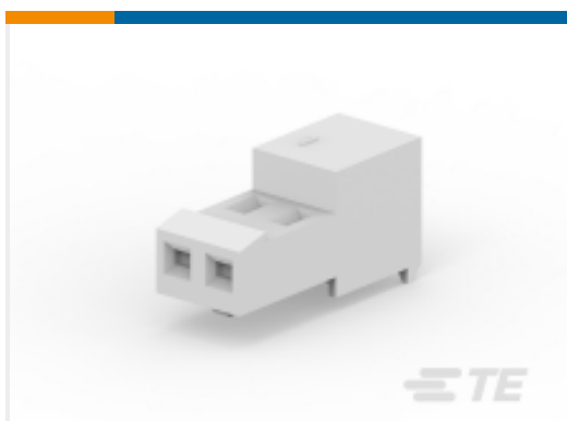
TE Part #4-640441-0 MTA Receptacle: Nylon, Tin Plated, 2.54 mm
