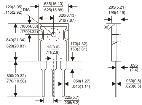
TO-247
