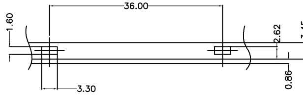
RECOMMENDED BRACKET CUTOUT
