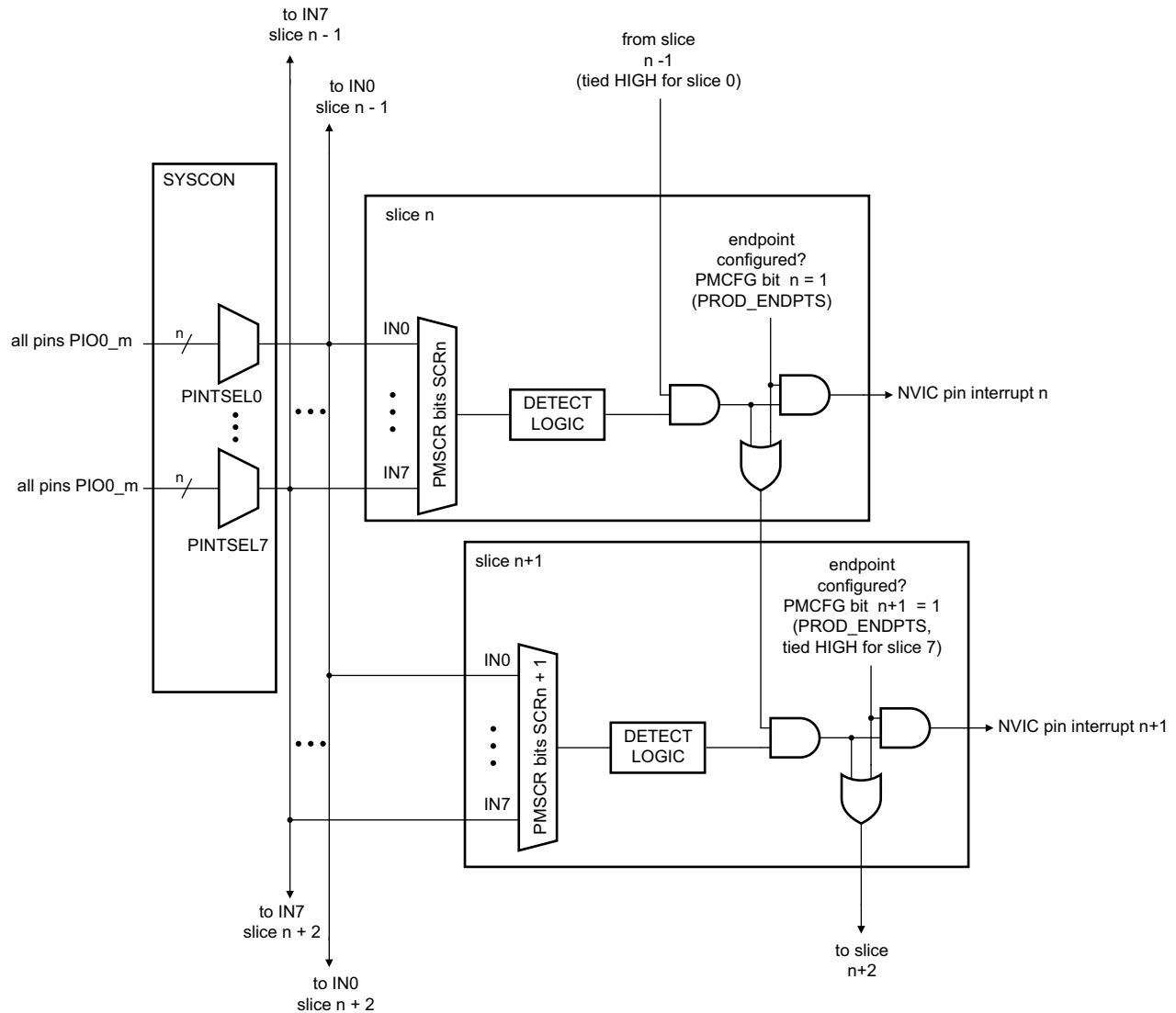
Fig 8. Pattern match engine connections
