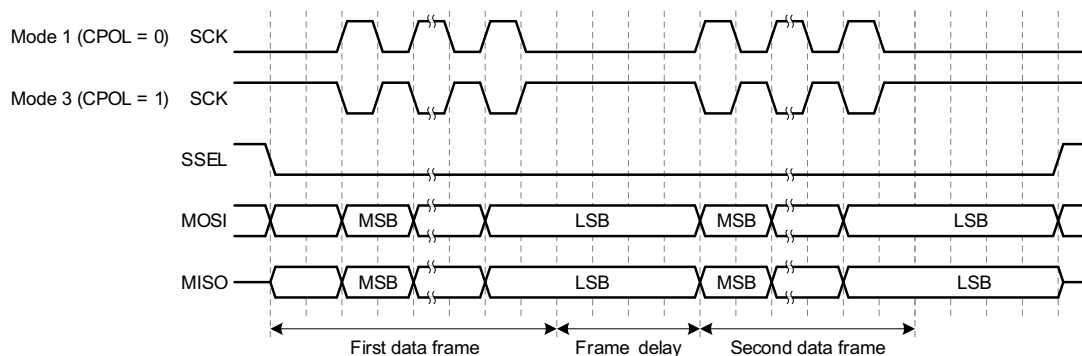
Fig 38. Frame_delay timing
