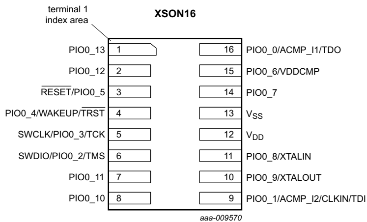
Fig 57. Pin configuration XSON16 package (LPC812M101JTB16)
