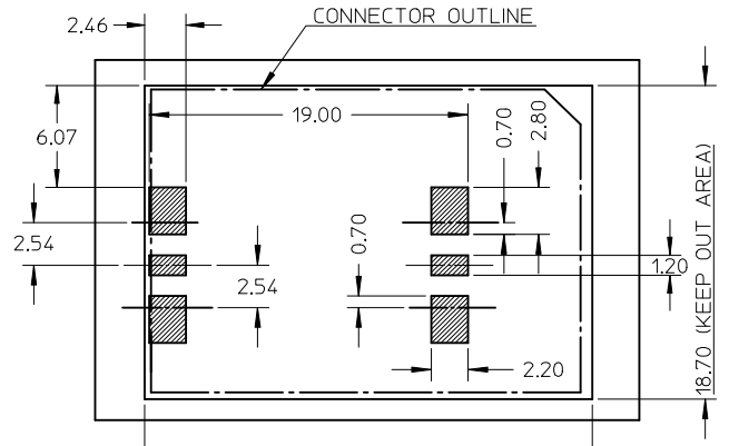
RECOMMENDED PCB LAYOUT(±0.05MM)
