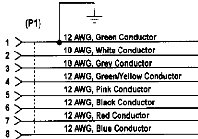
Wiring Diagram for 569659
