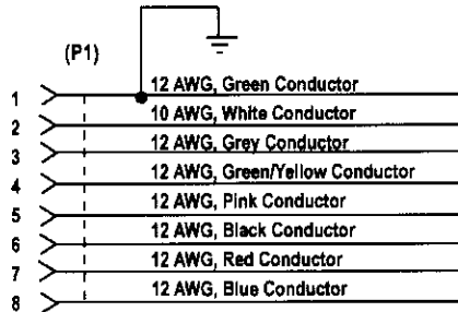
Wiring Diagram for 557653, 556148
