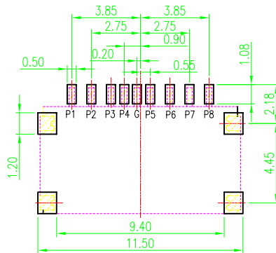
RECOMMEN P.C.BOARD LAYOUT GENERAL TOLERANCE ±0.05
