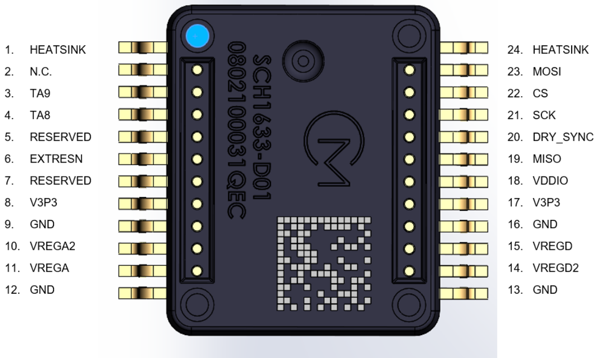
Figure 1 SCH16T-K01 pin layout
