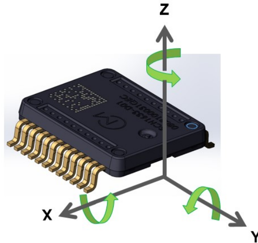
Figure 3 SCH16T-K01 measurement directions for gyroscope and accelerometer
