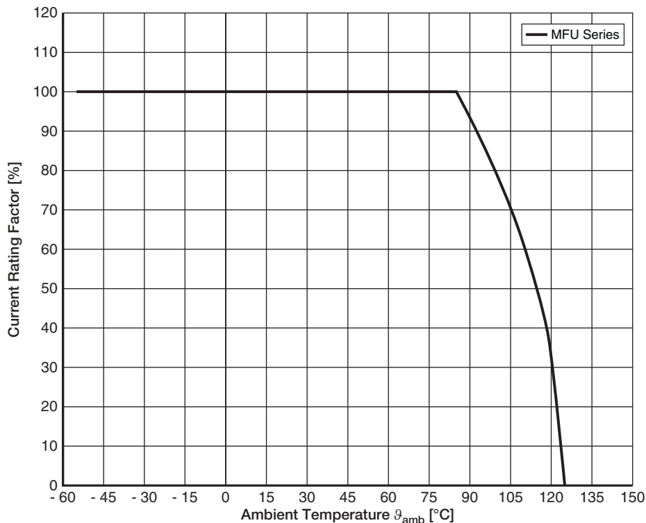
Current Rating Factor (1) vs. Ambient Temperature T_amb
