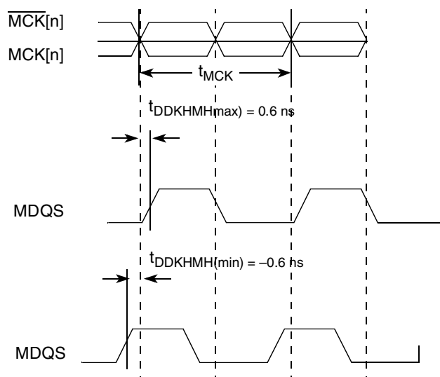
Figure 9. Timing Diagram for t_{DDKMH}
