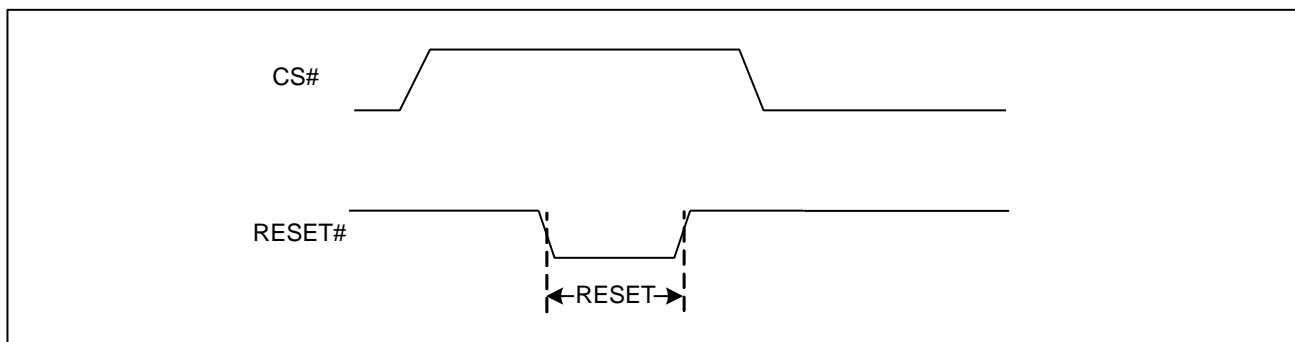
Figure 1 RESET Condition
