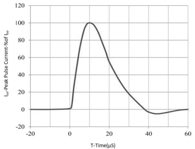
EC61000-4-5 Waveform( 8/20 \mu s pulse)
