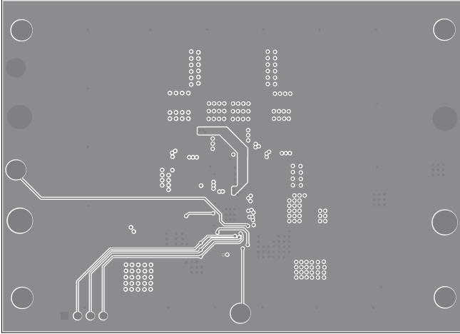
Figure 5: Middle Layer 3
