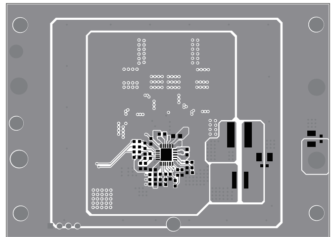
Figure 8: Bottom Layer
