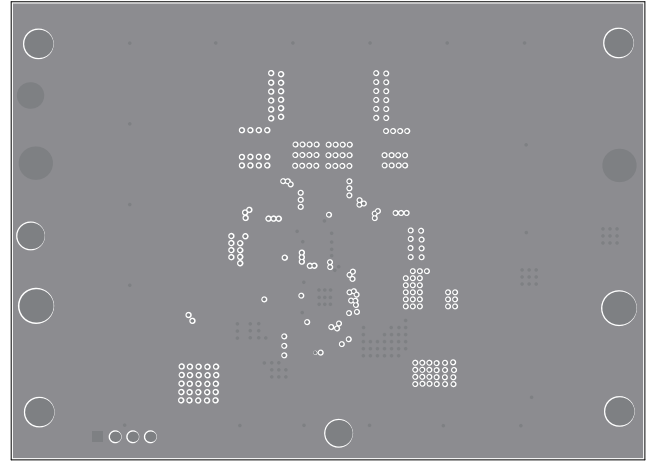
Figure 6: Middle Layer 4
