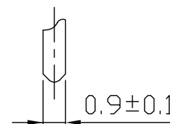
TERMINAL DETAIL
