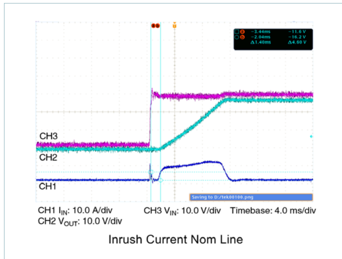
Figure 4 — Inrush limiting; inrush current with 3300μF external capacitance
