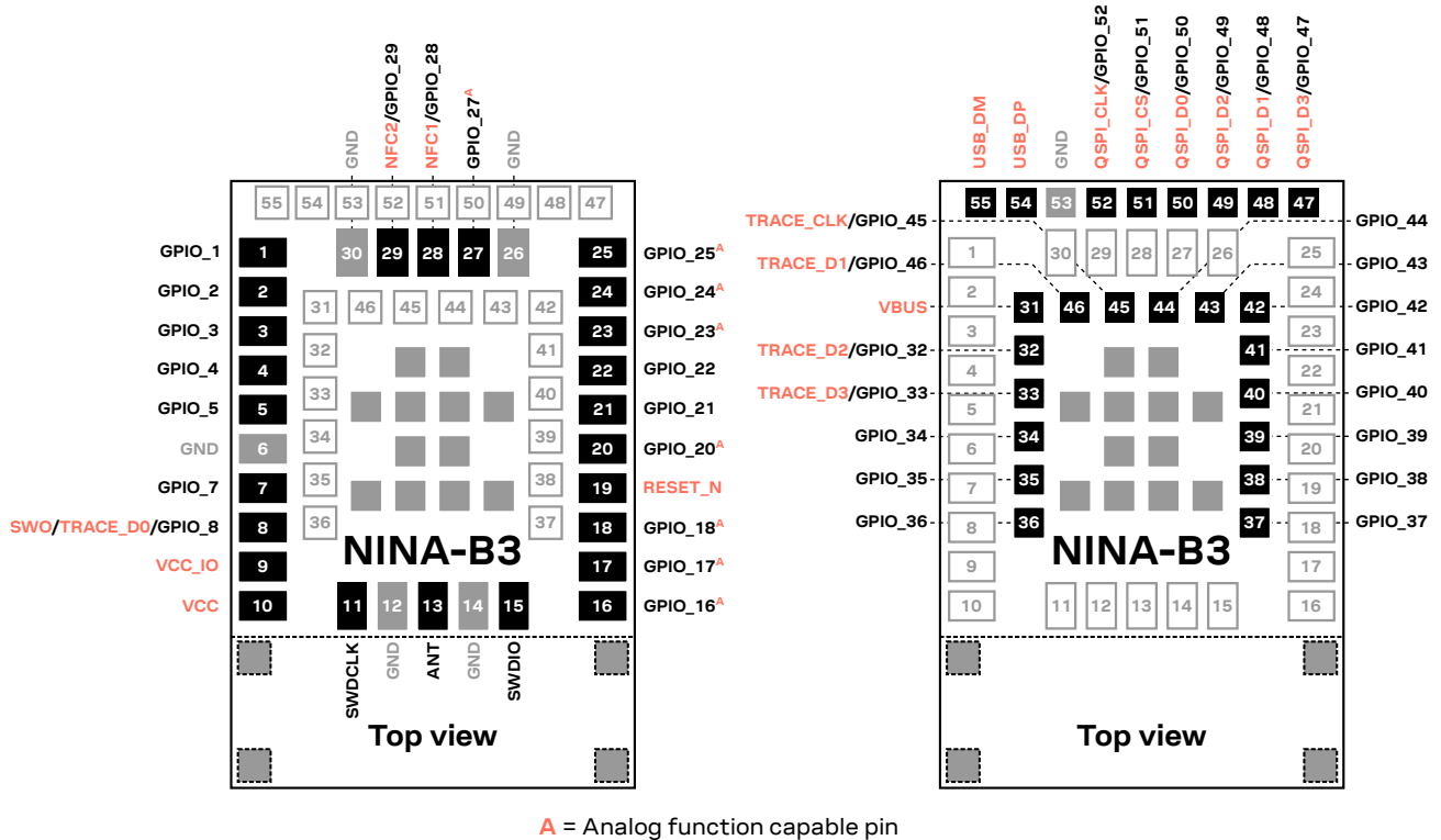
Figure 4: NINA-B30 series pin assignment (top view)
