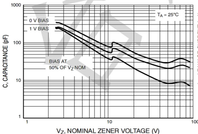
Figure 7. Typical Capacitance
