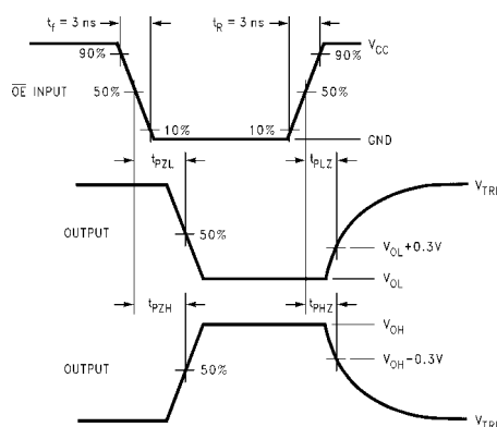
Figure 6. AC Waveforms
