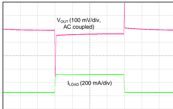
Time (50 \mu\text{s}/\text{div} ) V_{IN} = 3.8\text{ V} , no output capacitor, output current slew rate = 0.25\text{ A}/\mu\text{s}
