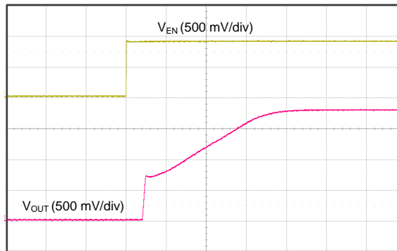
Time (100 \mu\text{s}/\text{div} ) R_L = 6.2\ \Omega , 1- \mu\text{F} output capacitor
