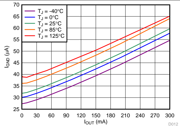
Figure 2. Ground Pin Current vs I_{OUT} and Temperature
