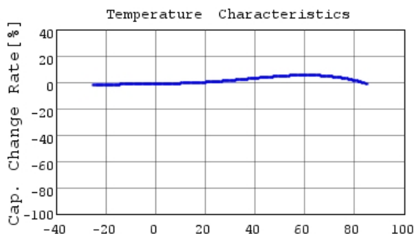
GRM31CB31E106KA75 C-Temp. capchange, DC0.0V,
