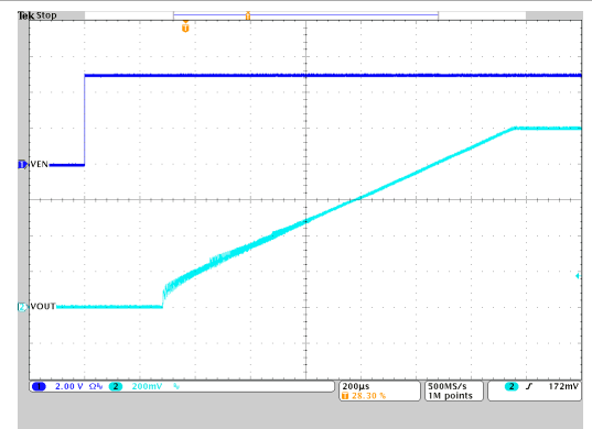
Figure 9-53. Start-Up Timing
