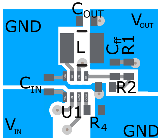
Figure 9-61. Example Layout
