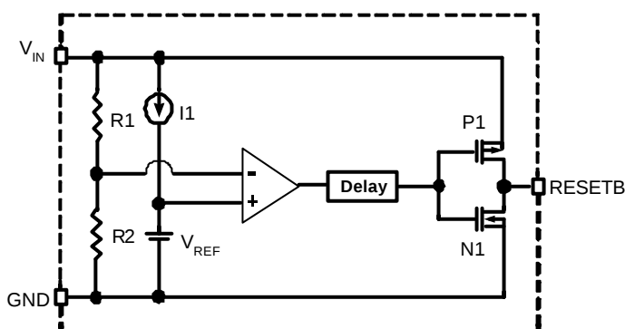
AME8500 with Push-Pull RESETB
