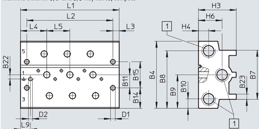
[1] Ports 1, 3 and 5: G1/4
