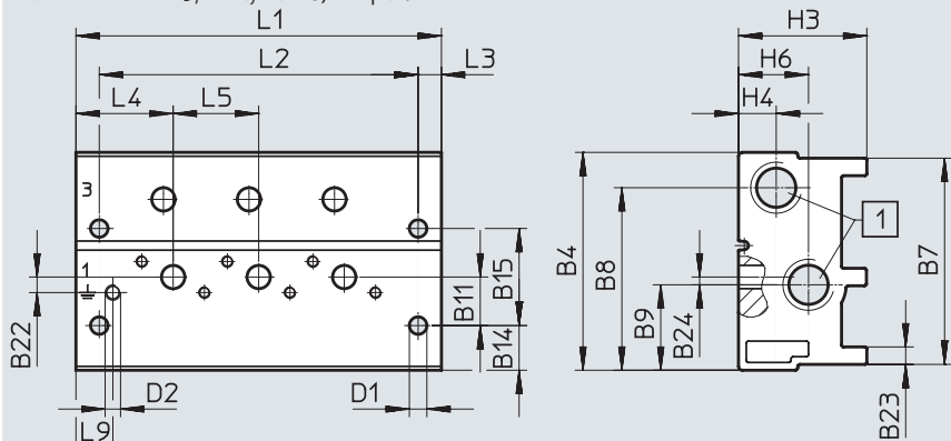
[1] Ports 1 and 3: G1/4
