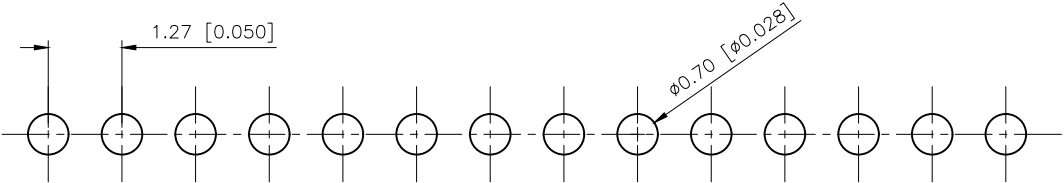
PCB LAYOUT
