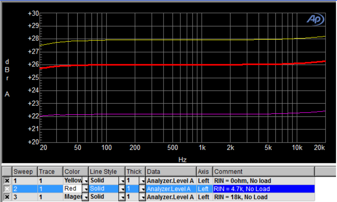
Frequency Respond
