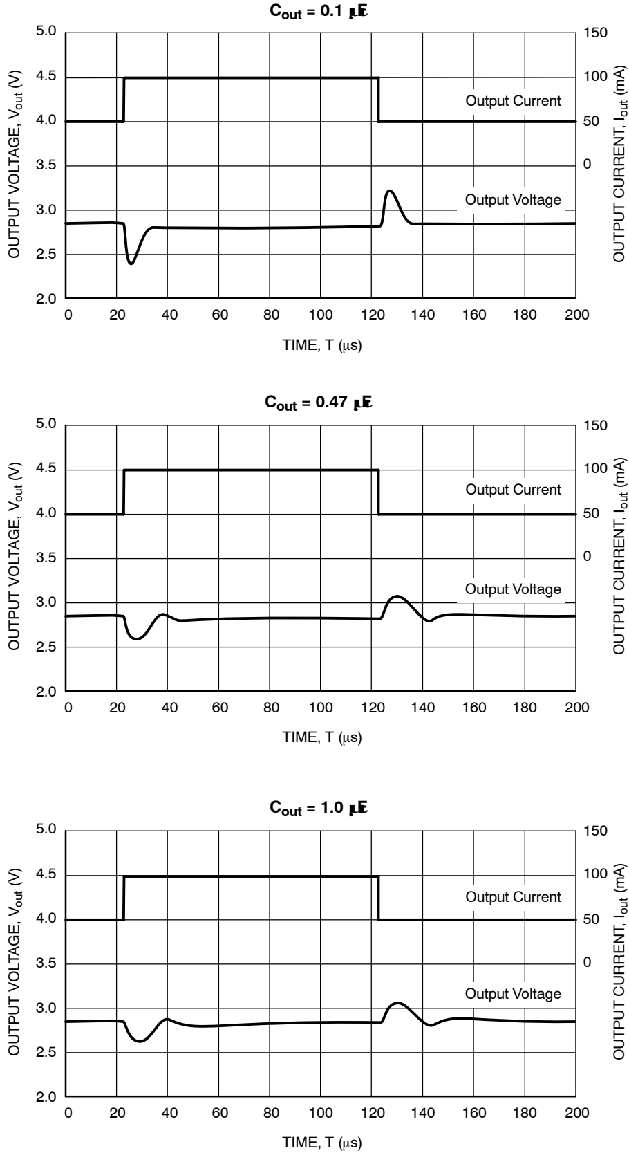
Figure 29. Load Transient Response (V out = 2.8 V, tr = tf = 5.0 μs, V in = 3.8 V)
