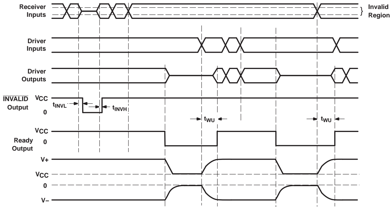
VOLTAGE WAVEFORMS
