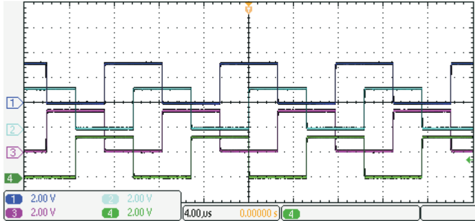
Figure 16. Multiphase PWMs
