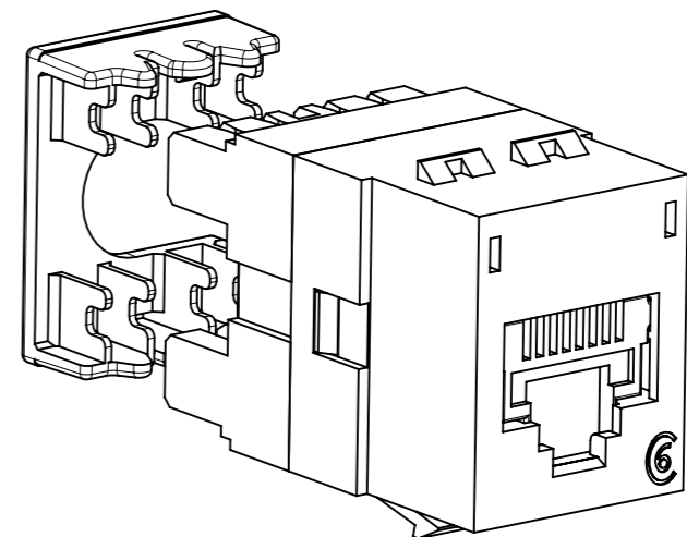
ISO VIEW
