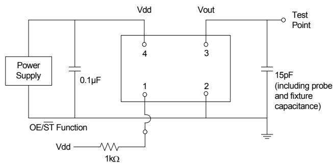
Figure 2. Test Circuit
