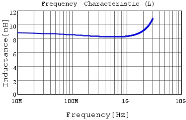
LQP03TN8N2H02 L
