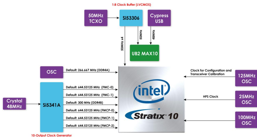
Figure 2-12 Clock circuit of the FPGA Board
