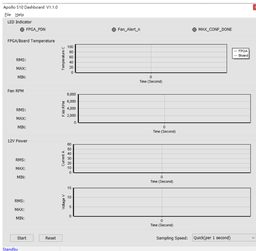
Figure 4-6 Dashboard GUI
