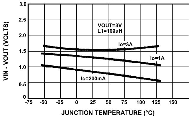
DROPOUT VOLTAGE
