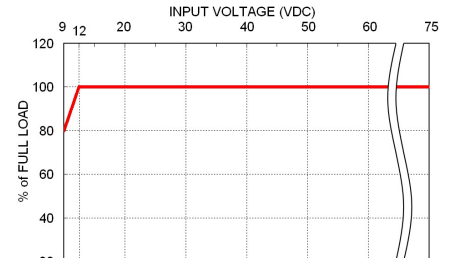
QAE100-36S05U Derating Curve vs. Input Voltage
