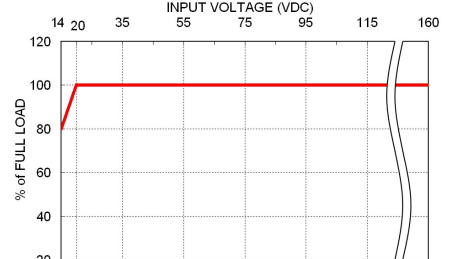
QAE100-72S05U Derating Curve vs. Input Voltage
