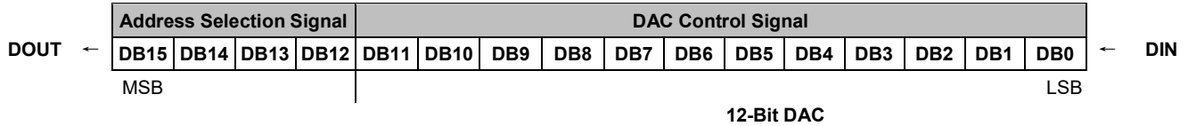
Figure 2. Serial Data
