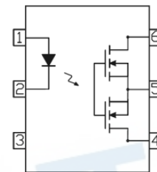
Pin Configuration
