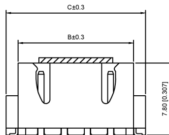
3P~16P Shape SCALE 1:1
