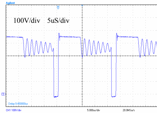
Vin=265V, Io=0.5A
