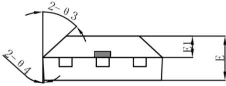
T092S 封装尺寸
