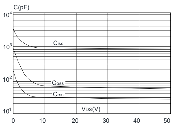
Figure 6: Capacitance Characteristics
