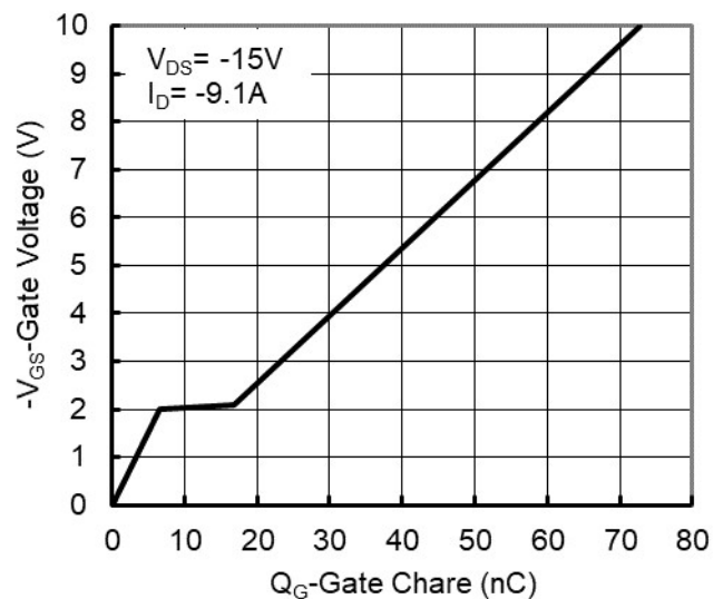
Figure 6. Gate Charge
