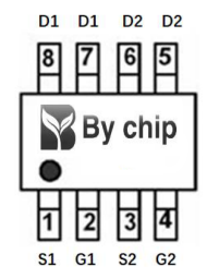
Pin Assignment
