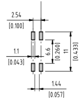
◆ P. C. B LAYOUT
