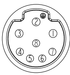
C1 & C2 Pin Assignments Front View
